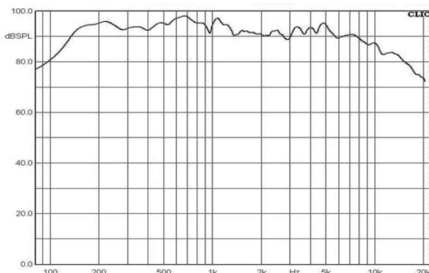
1.20.006 Médio Grave 8" Outdoor 200Wrms 4 ohms
