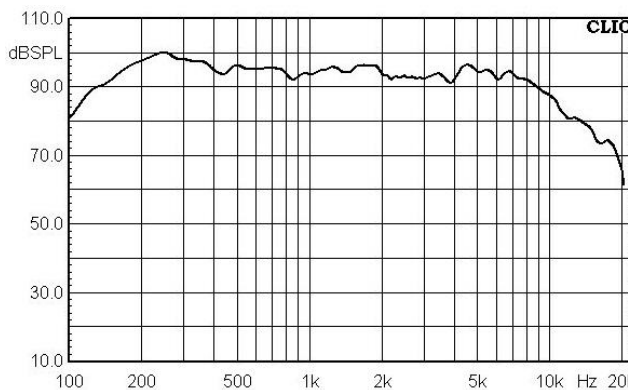
1.20.007 Médio Grave 8" Outdoor 200Wrms 8 ohms
