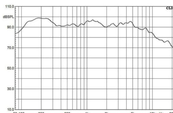
1.20.007 Médio Grave 8" Outdoor 200Wrms 8 ohms
