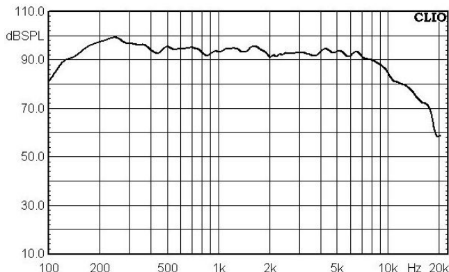
1.20.006 Médio Grave 8" Outdoor 200Wrms 4 ohms
