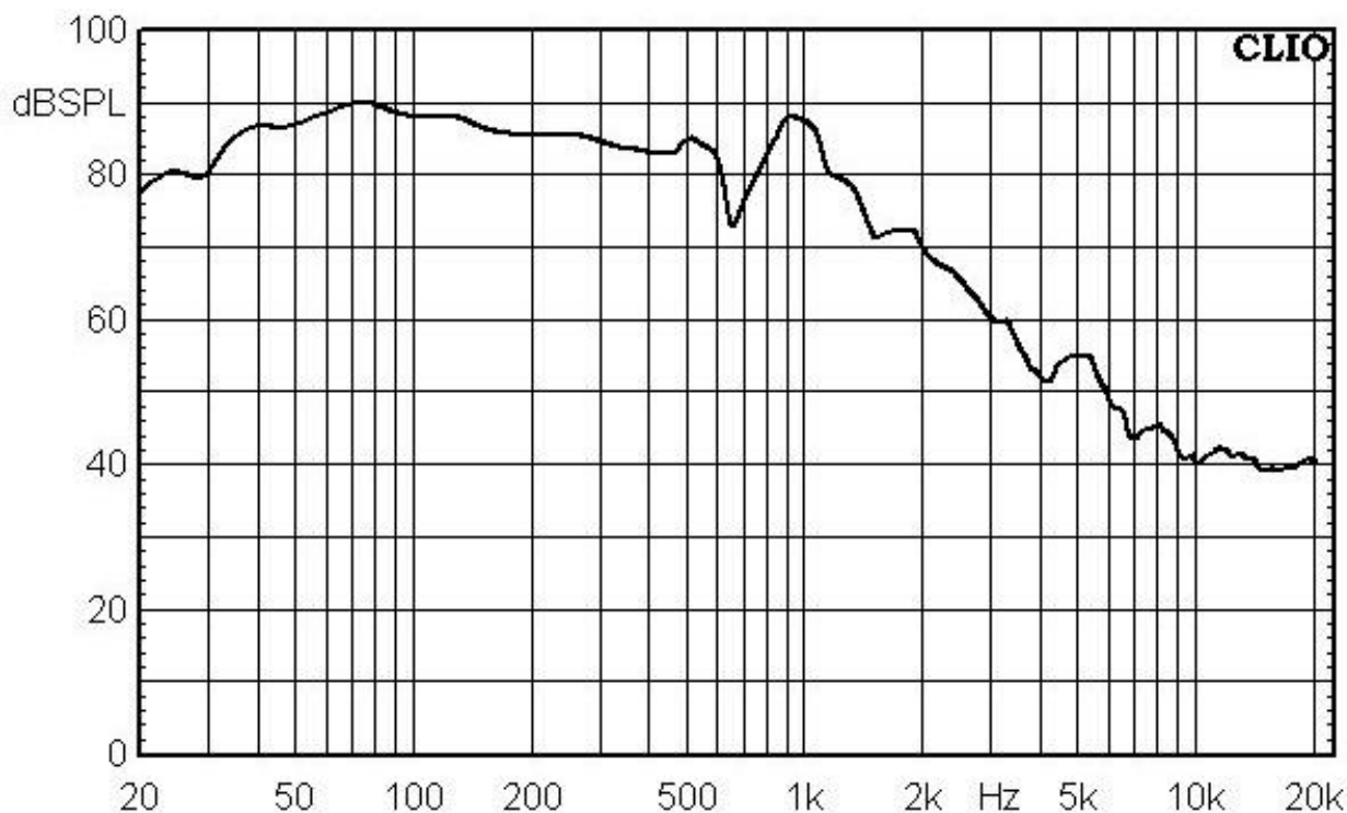
CURVA DE RESPOSTA / RESPONSE CURVE (1W/1m) ①②
